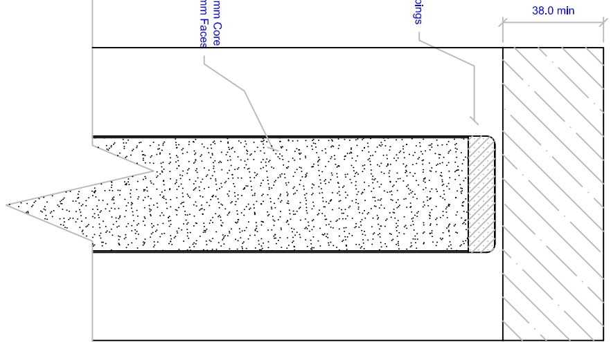
INT - DA01 Hanson & Beards 44mm Double Action Pivot Door with Frame Vertical Through Sectional Drawing Detail
